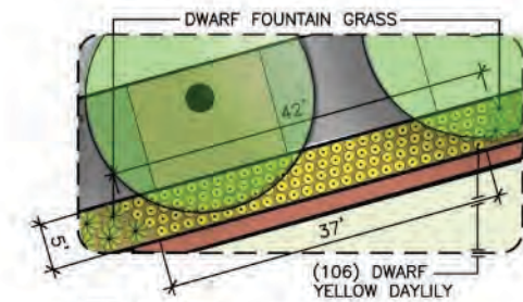
A05 1"=10'-0" 600 S. STATE STREET Poggemeyer Design Group
