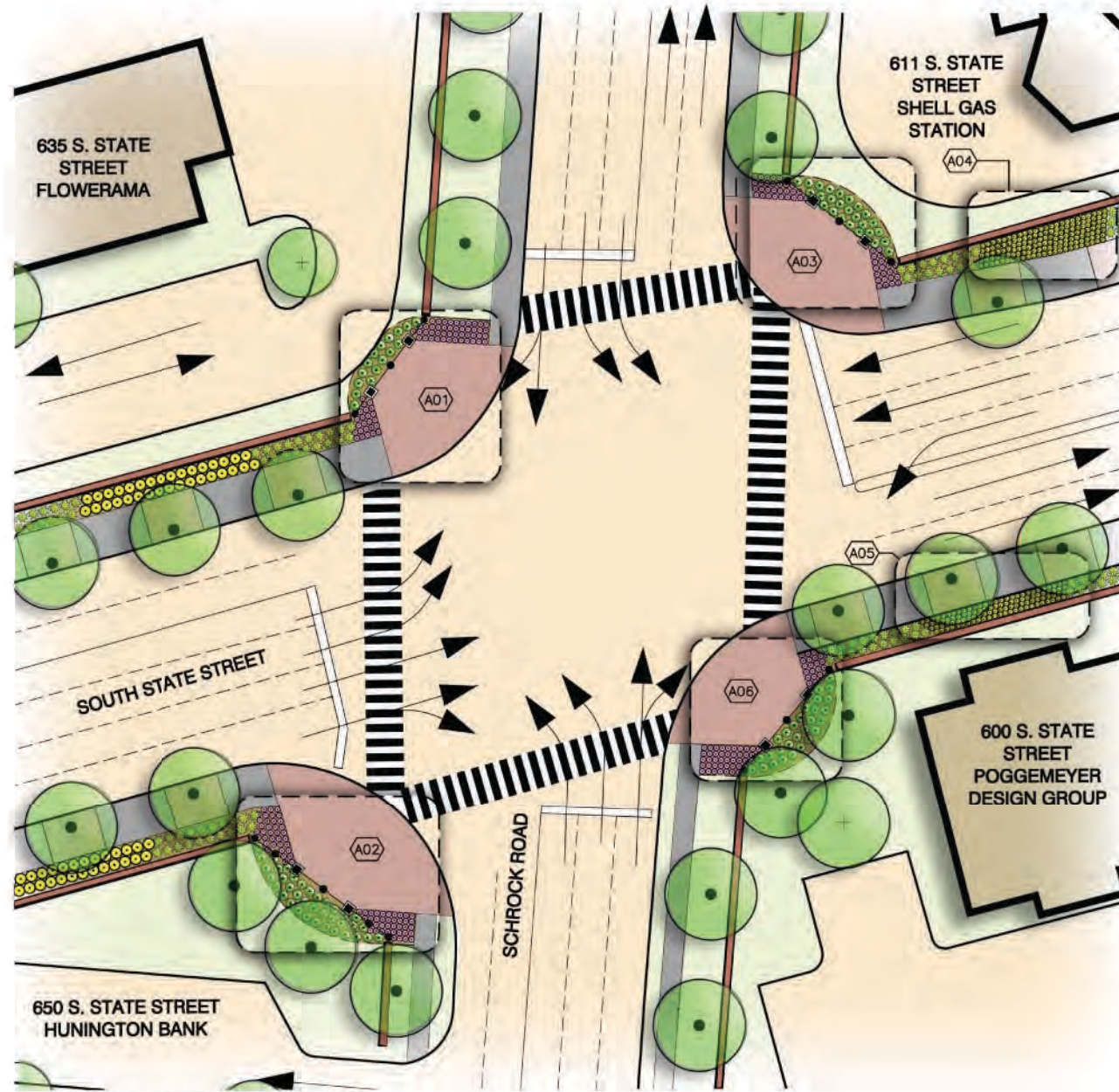
INTERSECTION NODE PROTOTYPE South State Street & Schrock Road 1"=20'-0"
