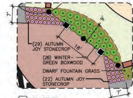
A03 1"=10'-0" NW CORNER OF INTERSECTION South State Street & Schrock Road
