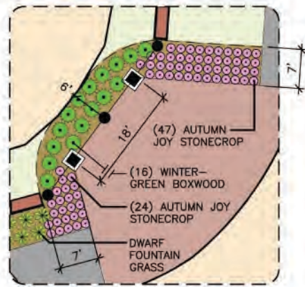
A01 1"=10'-0" SW CORNER OF INTERSECTION South State Street & Schrock Road
